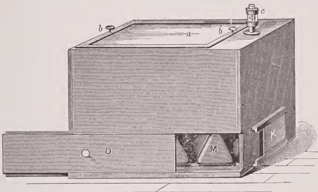
FIG. 66.—Modified Auvard incubator or couveuse : a , glass plate of the movable lid ( b ); c , ventilating tube containing small rotary fan; k , ventilating slide; m , hot-water cans; o , slide closing hot-air chamber.
